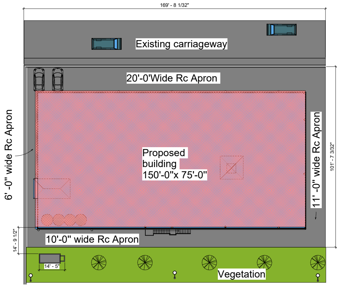
Site Plan
