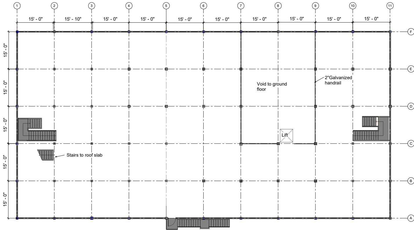
First Floor Layout
