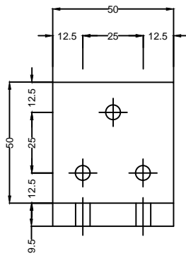
TYPICAL RAFTER TO TANK CONNECTION DETAIL B-B NTS
