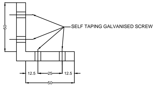
TYPICAL RAFTER TO TANK CONNECTION DETAIL B-B NTS
