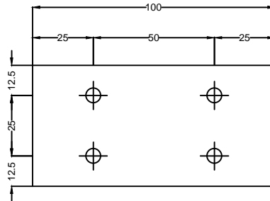
TYPICAL RAFTER TO RAFTER CONNECT DETAIL A-A NTS
