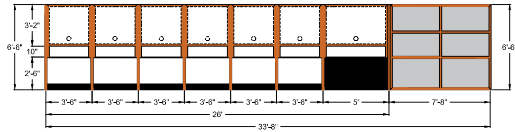
ELEVATION OF PARTITION (NEW SERVICE)
