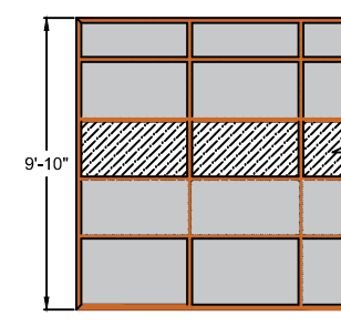
ELEVATION OF MANAGER AND COMMERCIAL OFFICER OFFICES (WITH PERSPEX)
